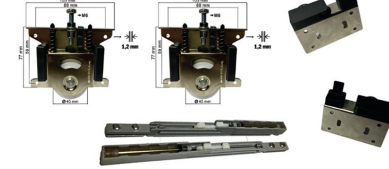
BSS-302 JUNIOR SET BSS-302 JUNIOR SET
